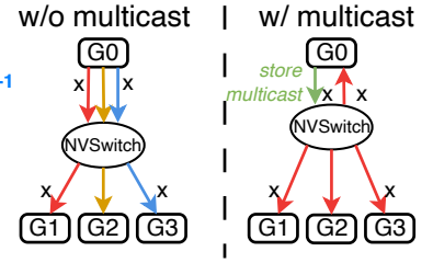
Figure 2: Operation of st_multicast .
