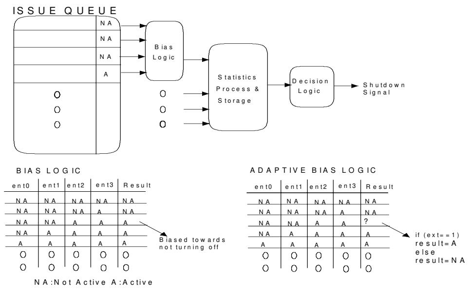
Fig. 3. High-level structure of shutdown logic and logic table for bias logic
