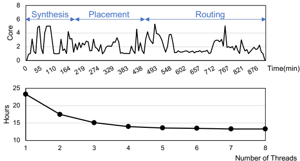
Figure 1: The upper figure shows the number of active CPU cores when implementing a CNN benchmark by Vivado (8 threads) on a 56-core server. The total implementation process takes about 14 hours, and with an average CPU utilization of 2.1 cores. The lower figure displays the runtime as we increase the number of threads.
