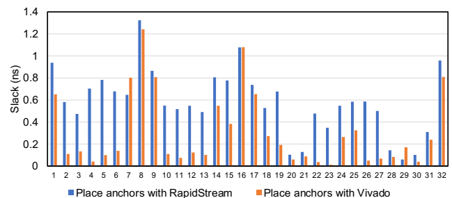
Figure 19: Post-placement slack between using the Vivado placer or the min-cost matching placer for anchor placement.
