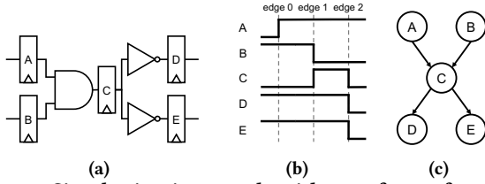
Figure 3: Simple circuit example with waveform of register outputs and register connection graph.
