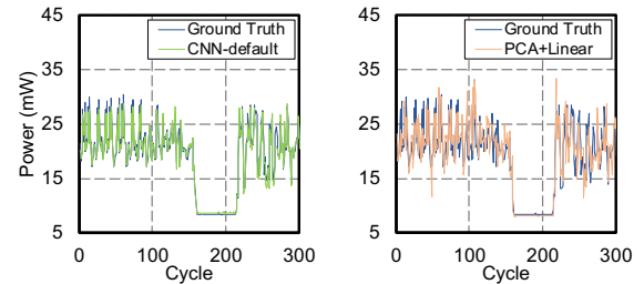
Figure 7: Ground truth vs. CNN-default and PCA+Linear for RISC-V — Showing 300 cycles from the dhrystone benchmark. the two-dimensional space. This problem itself is an interesting research direction, and we leave it for future work.
