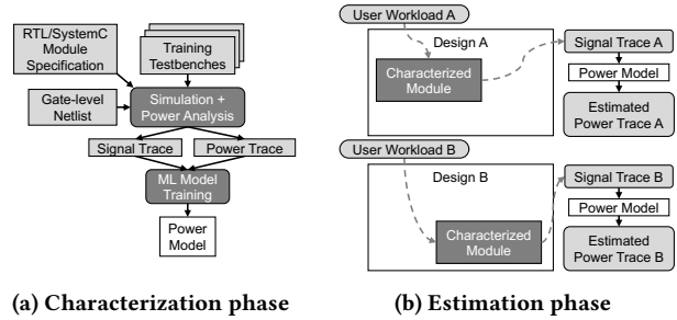
(a) Characterization phase (b) Estimation phase Figure 2: Two phases of the PRIMAL workflow – Power models are trained once per module , then used across different workloads and in different designs that instantiate the module.
