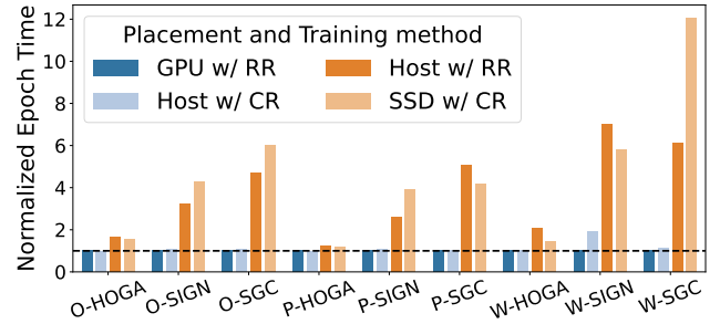
Figure 14. Placement influence on epoch time — The first item in the legend represents input data location while the second item represents the training method, with RR standing for SGD-RR and CR for chunk reshuffling.
