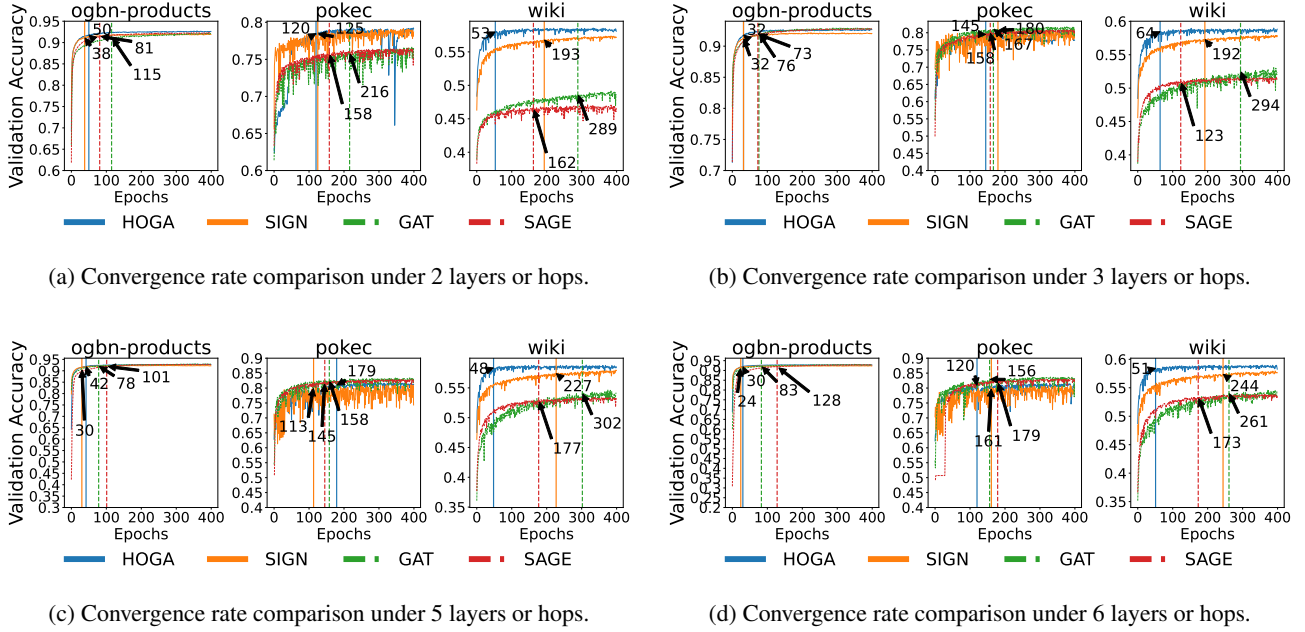
Figure 10. Convergence rate comparison among MP-GNNs and PP-GNNs— The number in the plot denotes the convergence point where 99% of peak validation accuracy is reached.
