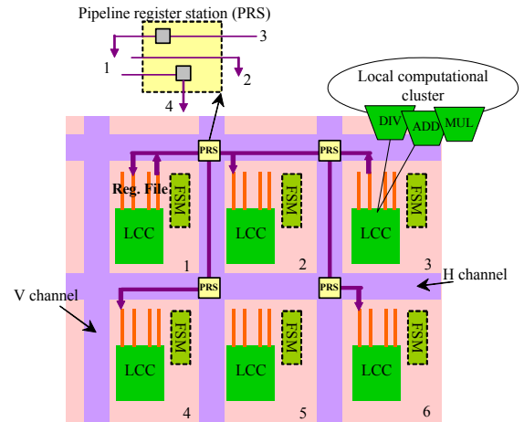
Figure 2. A 2x3 island-based RDR-Pipe micro-architecture.
