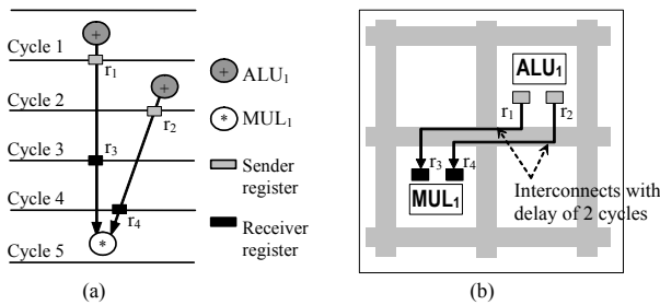
Figure 1. Illustration of the wiring overhead in RDR (a) Scheduled and bound CDFG, (b) RDR layout.
