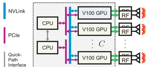
Fig. 4. Overview of the experimental platform with up to eight Tesla Volta GPUs and high speed NvLink GPU-to-GPU interconnect [17]. The uppermost GPU is the master GPU that collects results from other GPUs, performs centralized computations for PD-WF, and broadcasts the transmit vectors \mathbf{s}[k] for FD-WF or the whitened vectors \mathbf{z}[k] for PD-WF to other GPUs.
