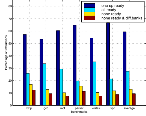
Figure 3: Percentage of instructions with various numbers of operands available on dispatch. Also shown is the percentage of cases in which neither source operand is available and where the source operand IDs are associated with different banks.
