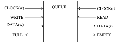
Figure 2. Queue structure
