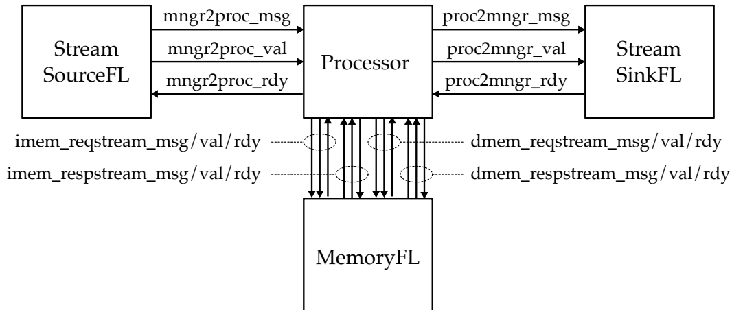
Figure 2: Processor System – The processor is integrated with a source, sink, and memory for testing and evaluation.
