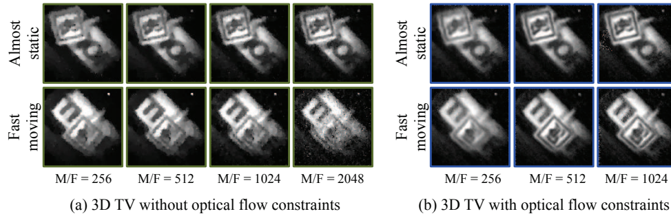
FIG. 16. Comparison of recovered videos with and without optical-flow constraints. Data was collected with a SPC operating at 10,000 Hz with a SWIR photodetector. A total of M = 16,384 compressive measurements were obtained at a DMD resolution of 128 \times 128 . In each case, we show multiple reconstructions with different number of compressive measurements associated with each frame. That is, in each instance, the number of recovered frame F is chosen to satisfy the target M/F value. (a) Reconstructions without optical flow constraints. The top row shows the pendulum at one end of its swing where it is nearly stationary. The bottom row shows the pendulum when it is moving the fastest. As expected, increasing the number of measurements per frame, M/F , increases the motion blur significantly. (b) In contrast, use of optical flow preserves the quality of results. The visual quality peaks at M/F = 512 (see supplemental videos).
