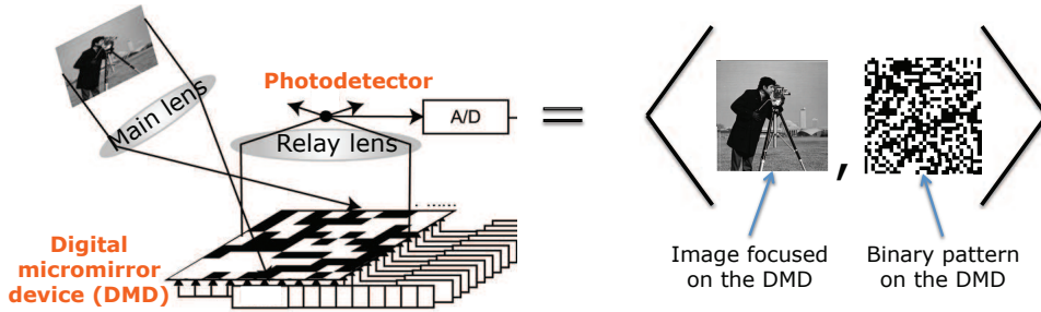
FIG. 3. Operation principle of the single pixel camera (SPC). Each measurement is the inner-product between the binary mirror-orientation patterns on the DMD and the scene to be acquired.
