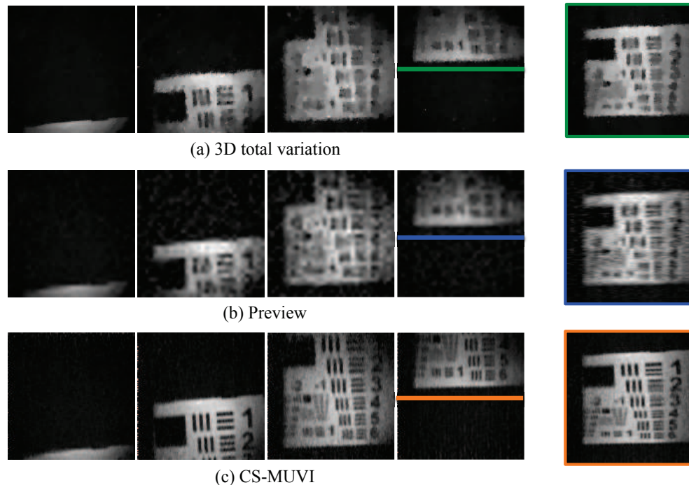
FIG. 17. Resolution chart. Reconstruction results on a translating resolution chart at a compression ratio of 32\times . In each row, we show frames from the recovered video as well as its xt slice in the color coded box in the last column.
