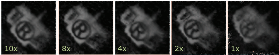
FIG. 20. Performance for varying scene illumination levels. We controlled the total light level in the scene by controlling the light throughput of the illumination sources. Shown above are results at different scene light levels—each case calibrated by the multiple of the minimum light level. In each case, we show one frame of the recovered video; the instant corresponding to the pendulum swinging at maximum speed. The performance degradation of the algorithm is graceful with only little artifacts.
