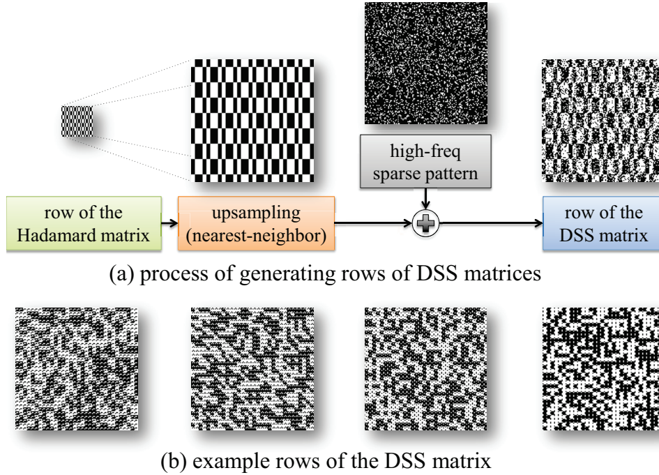
FIG. 7. Generating DSS patterns. (a) Outline of the process in (5.1). (b) In practice, we permute the low-resolution Hadamard for better incoherence with the sparsifying wavelet basis. Fast generation of the DSS matrix requires us to impose additional structure on the high-frequency patterns. In particular, each sub-block of the high-frequency pattern is forced to be the same, which enables fast computation via convolutions.
