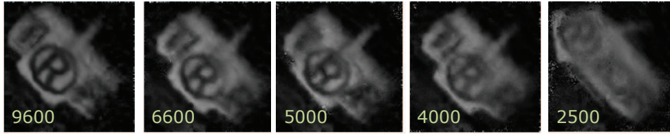
FIG. 19. Performance for varying speed. We slowed down the operating speed of the SPC to indirectly increase object speed. The operating speed of the SPC is overlaid on top of the recovered video. Shown is a single frame from each recovered video; the instant corresponding to the pendulum swinging at maximum speed.
