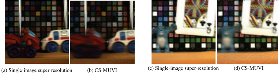
FIG. 12. Comparisons to the single-image super-resolution algorithm of [41]. Shown are results on two high-speed videos. (a,c) We use a low-resolution Hadamard matrix to sense a low-resolution image with 64 \times 64 pixels and subsequently, super-resolve them 4\times . (b, d) We use DSS matrices instead of low-resolution Hadamard to obtain the CS-MUVI results. Both algorithms have the same measurement rate. We observe that performance of CS-MUVI is similar to that of the super-resolution algorithm.
