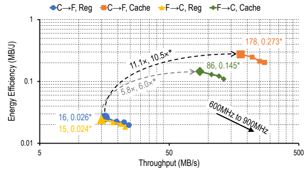
Fig. 7: CPU-FPGA Communication Throughput and Energy Efficiency at Different System Clock Frequency
