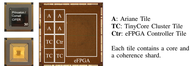
Fig. 1: CIFER Package and Die Photos
