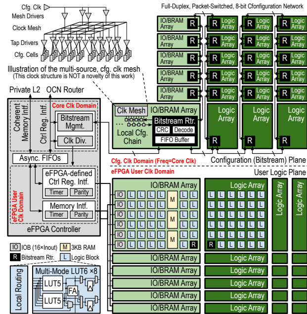
Fig. 3: CIFER eFPGA Architecture
