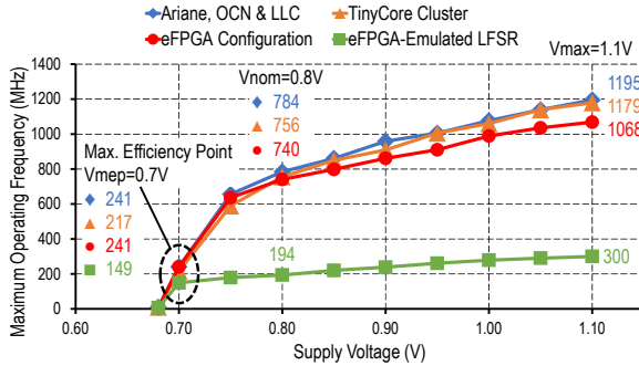
Fig. 5: Max. Operating Frequency vs. Supply Voltage
