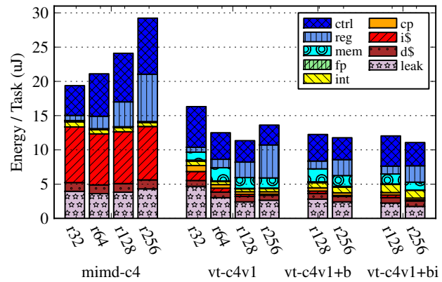
(b) Energy Breakdown for bsearch-cmv
